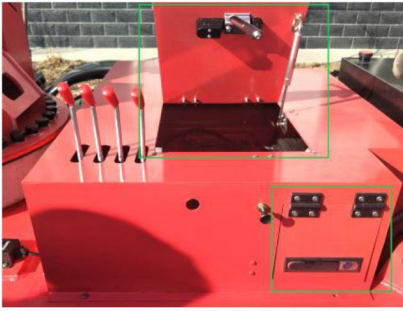
Special Design Cambered Joint Precise Joint Connection/Clamps
